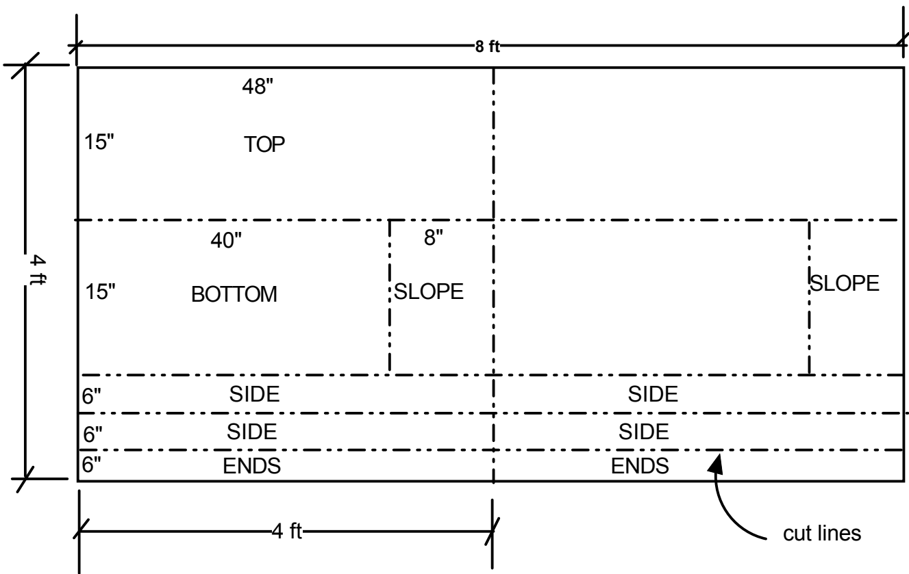
CUTTING PLAN FOR 8ft X 4ft PLY SHEET materials for 2 barges
